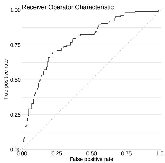
Figure 13.9: Graphical summary of model performance using the Receiver Operator Curve (Section 3.4).
