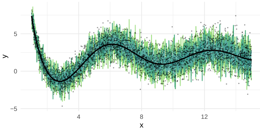
Figure 14.17: Results of quantile regression with GAM. 90%-prediction interval in green and 50%-prediction interval in blue. The black line is the underlying function.
