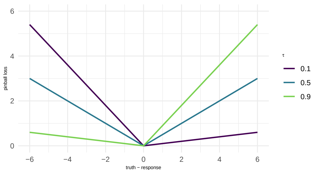
Figure 14.16: Values of the pinball loss function for different quantiles.
