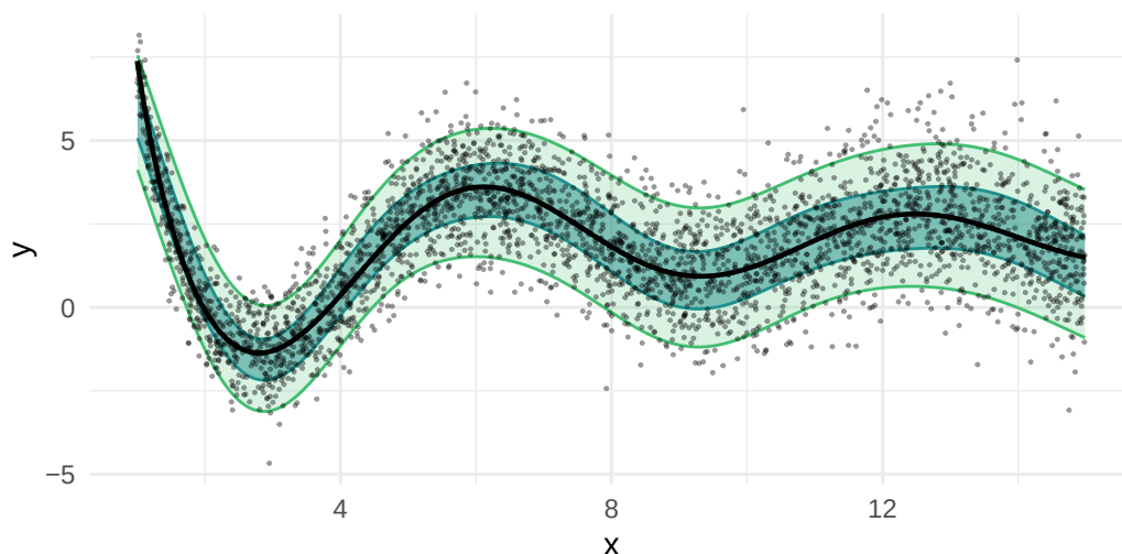
Figure 14.18: Results of quantile regression with GAM. 90%-prediction interval in green and 50%-prediction interval in blue. The black line is the underlying function.
