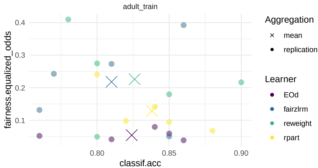
Figure 15.2: Comparison of learners with respect to classification accuracy (x-axis) and equalized odds (y-axis) across (dots) and aggregated over (crosses) folds.
