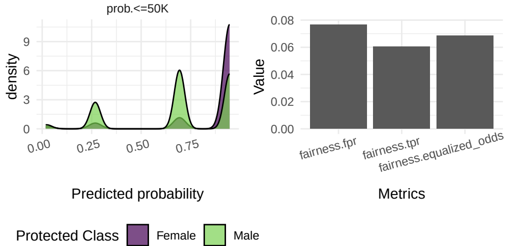
Figure 15.1: Fairness prediction density plot (left) showing the density of predictions for the positive class split by “Male” and “Female” individuals. The metrics comparison barplot (right) displays the model’s scores across the specified metrics.
